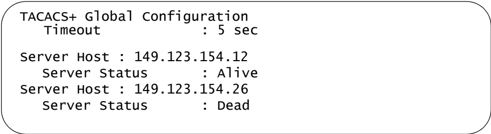
Figure 222. SHOW TACACS Command
