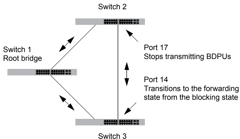
Figure 114. Loop Guard Example 2
