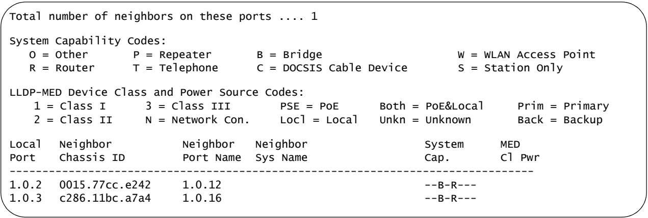
Figure 185. SHOW LLDP NEIGHBORS INTERFACE Command
